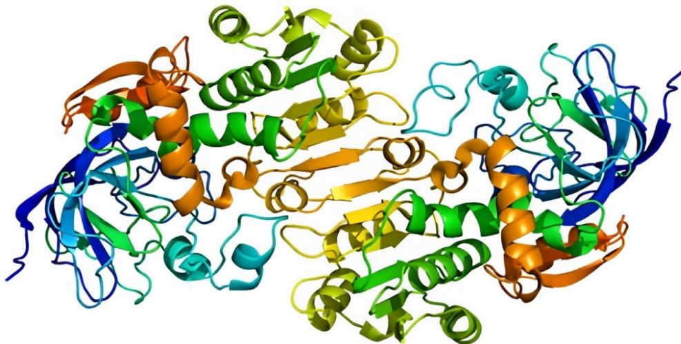
Fig. 2.4: Soil Dehydrogenase Model (Adapted from Protein Data Bank: 1m6h; (Sanghani et al. , 2002).
