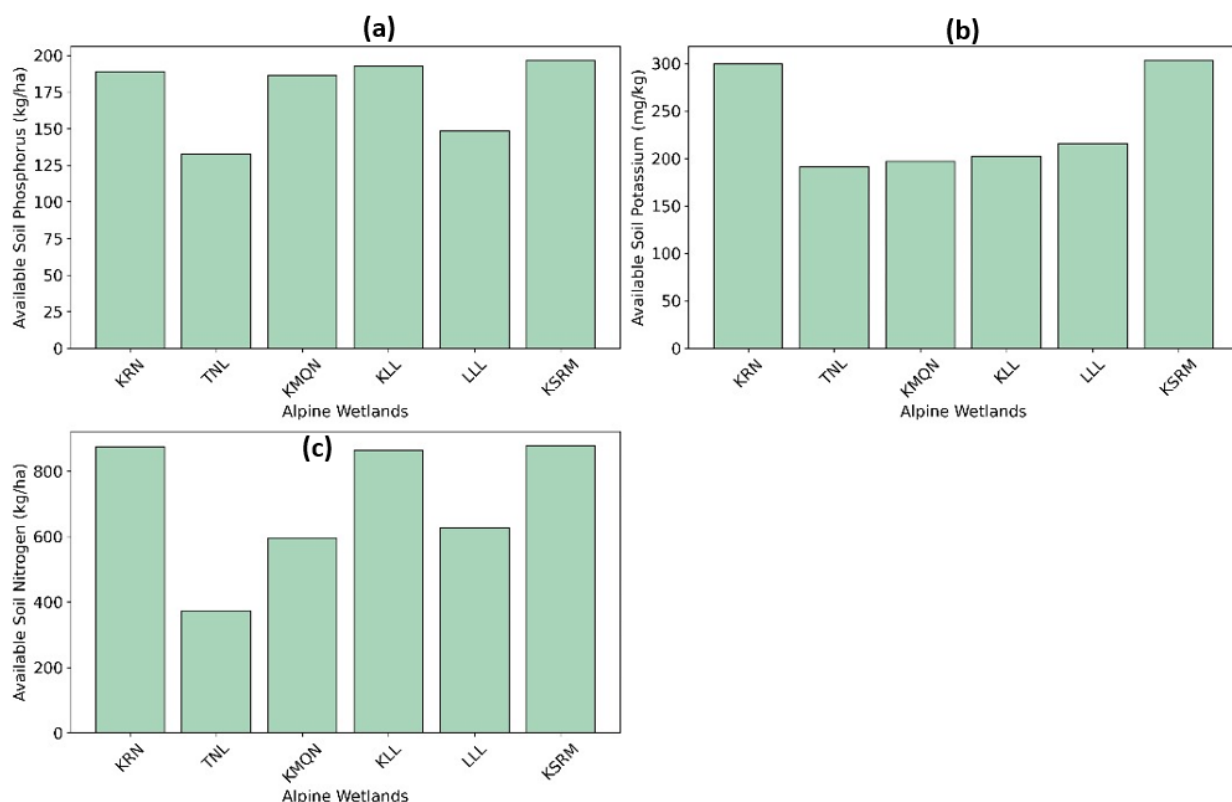
Figure 4.3: Impact of altitudinal variation on Phosphorus (a), Potassium (b) and Nitrogen (c) at 0-15 cm soil depth. KRN= Khorong (2500-2550m asl); TNL= Tenesolo (2552-2600m asl); KMQN= Khamoqana (2839-2880m asl); KLL= Khalong-la-Lichelete (2891-2995m asl); LLL= Lets'eng-La-Likhama (3040-3080m asl); KSRM=Koting-sa-ha Ramosetsana (3087-3155m asl).
