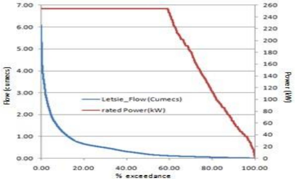
Figure 22: power curve for Letseng-la-Letsie
