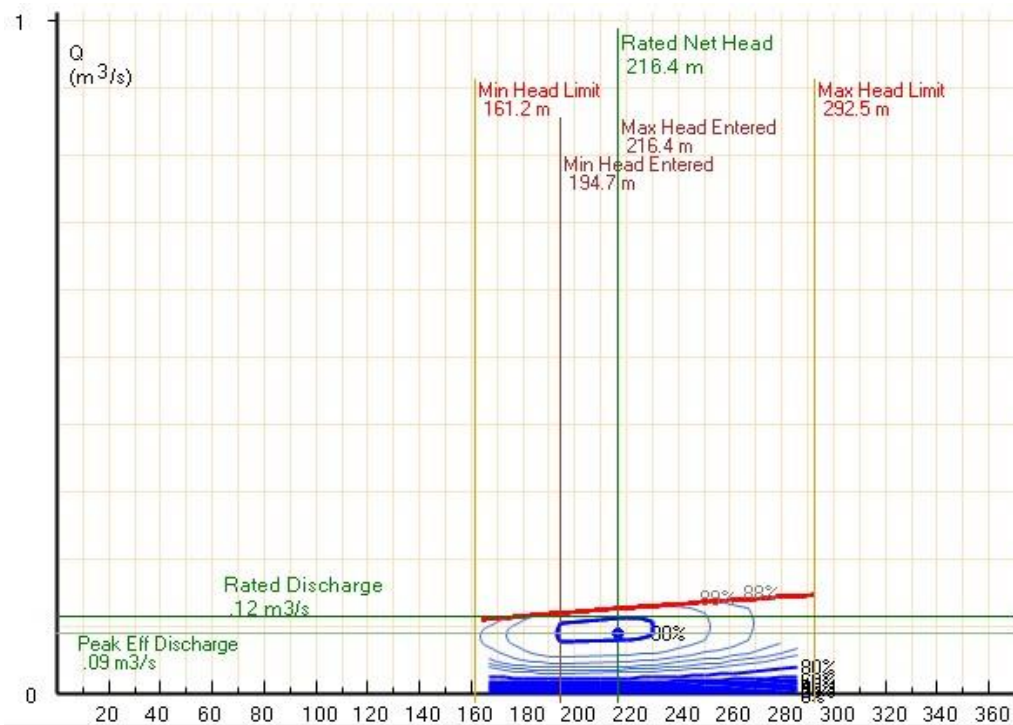
Figure 42: Letseng-la-Letsie Pelton Turbine Hill curve
