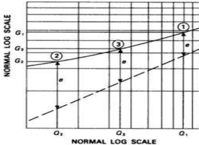
Figure 2: Stage Gauge curve determined by Johnson's method
