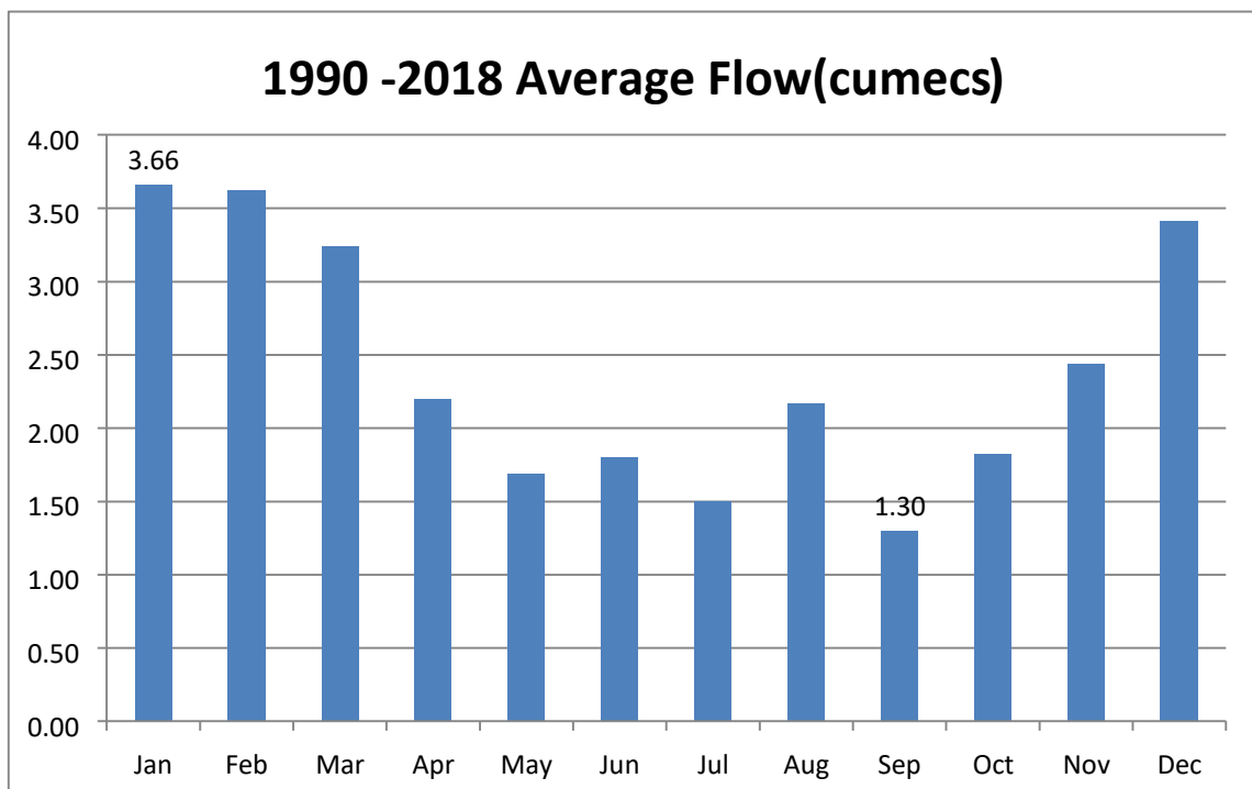
Figure 14: Quthing River Monthly Average flow rates
