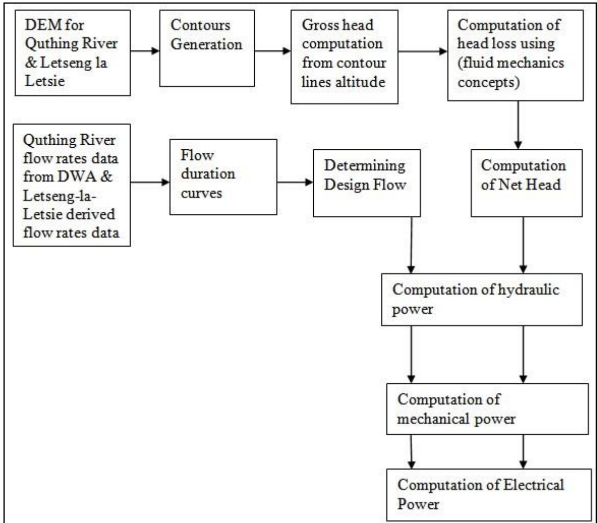
Figure 7: Methodology Flowchart
