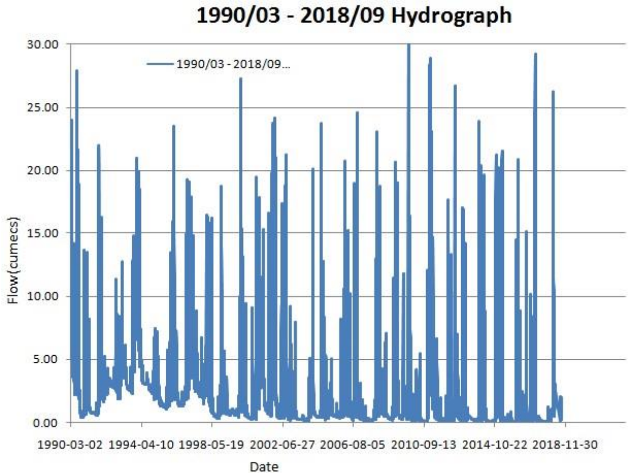
Figure 12: hydrograph of Quthing River (1990/03 – 2018/09)
