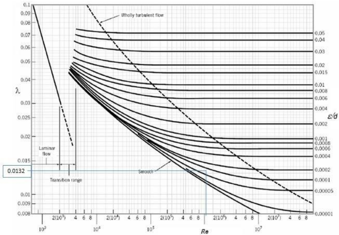
Figure 18: Friction factor for Quthing River [Source: ResearchGate]
