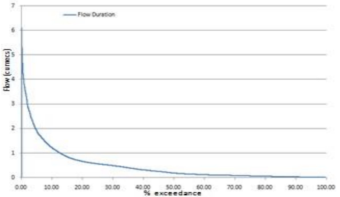
Figure 17: Letseng-la-Letsie FDC
