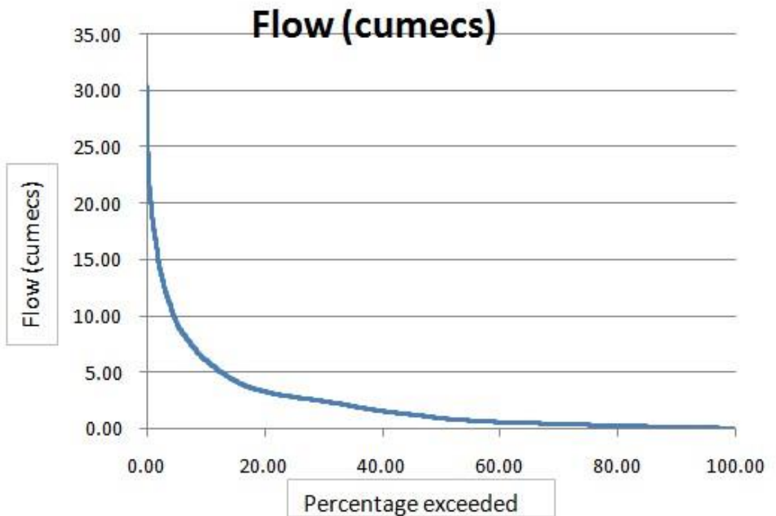
Figure 17: Letseng-la-Letsie FDC
