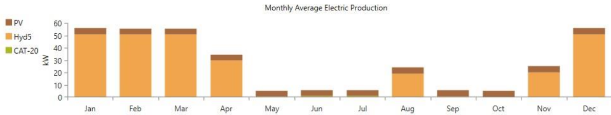
Figure 25: Electricity production results for Mashai hybrid system
