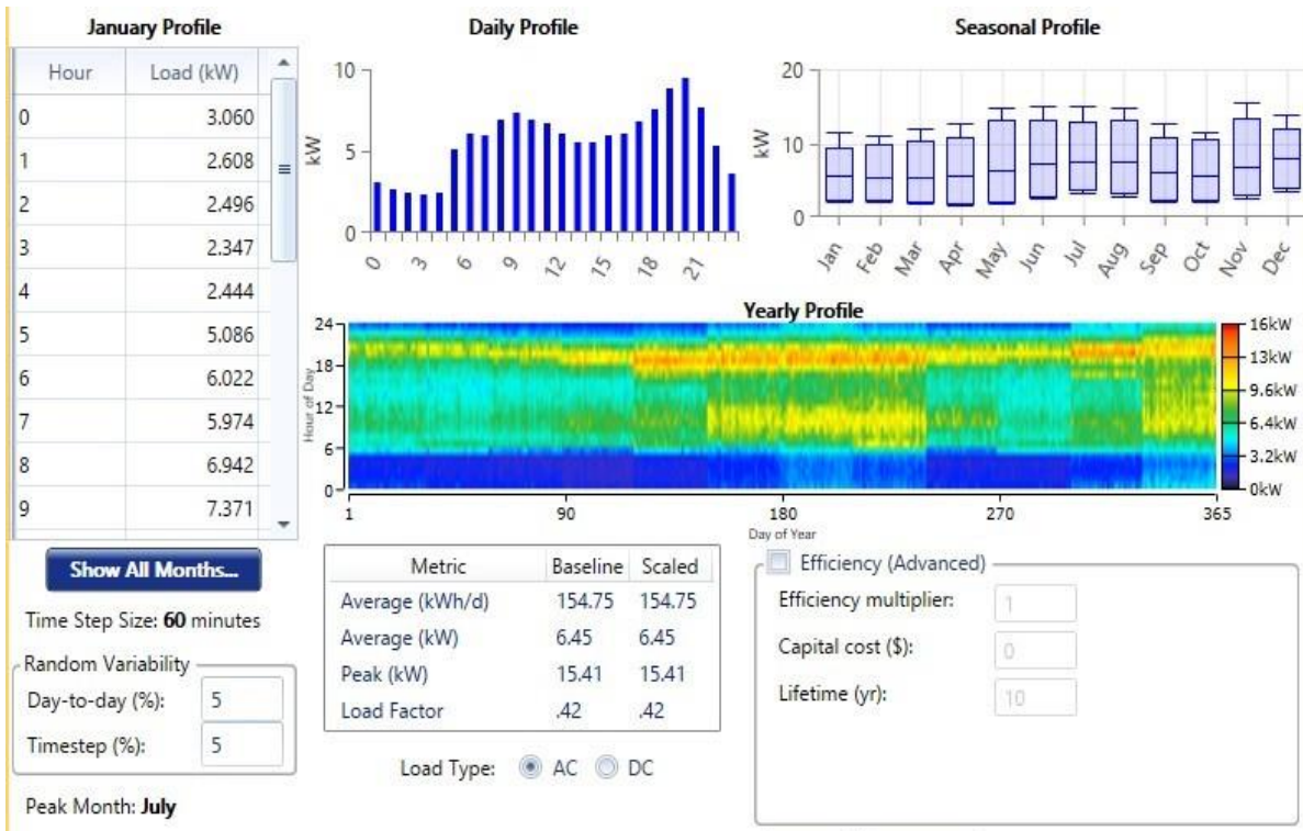
Figure 20: Daily, seasonal and yearly load profile for Mashai
