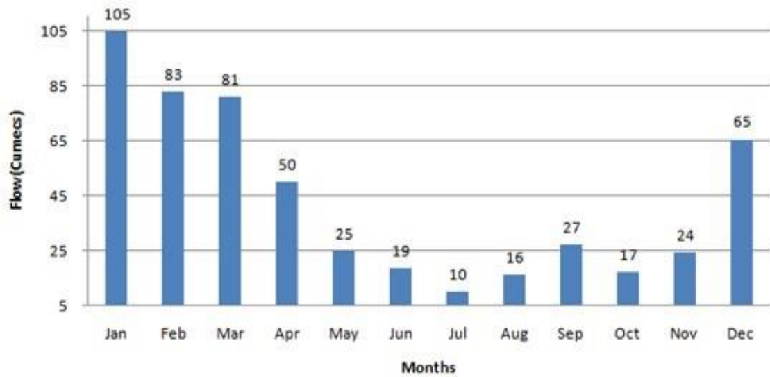
Figure 10: Monthly Average flow rates for Sehonghong- Senqu River at KomaKoma
