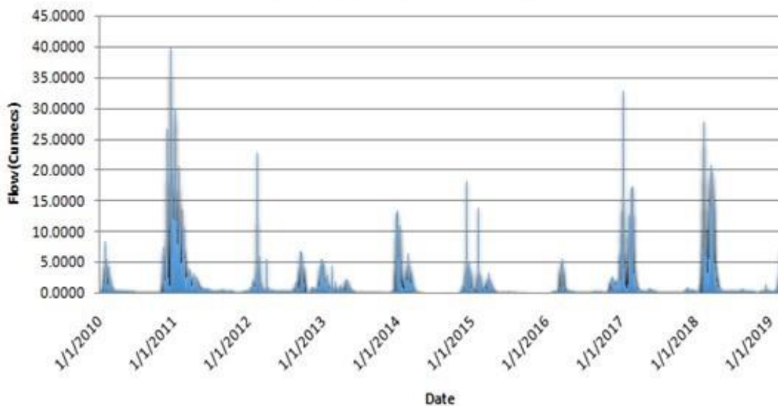
Figure 8: Hydrograph for Mashai( Mashai River at St Theresa)
