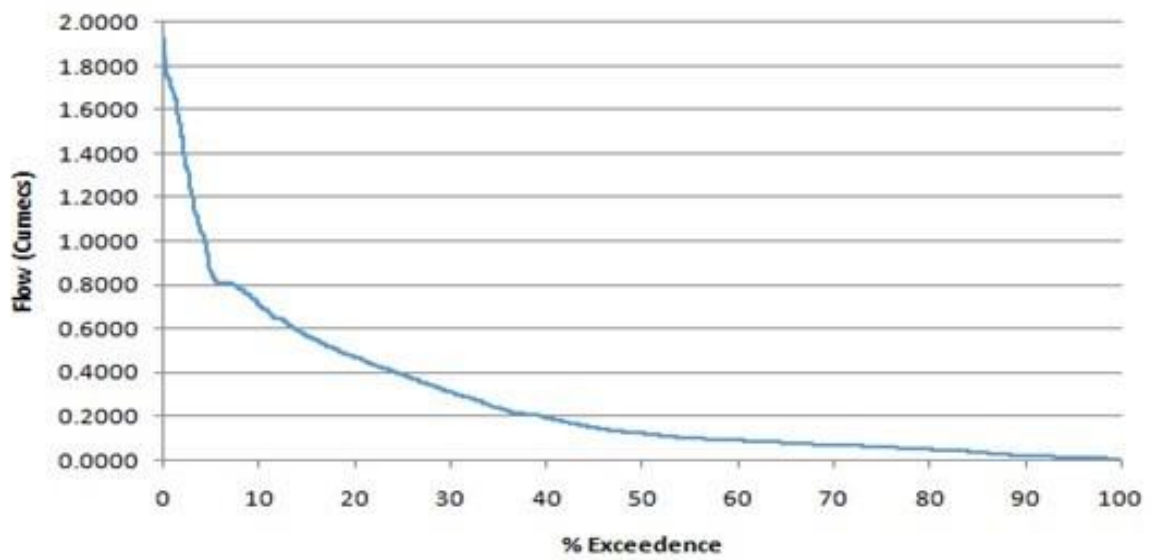
Figure 13: Flow duration Curve for Sehonghong (Senqu River at Sehonghong)
