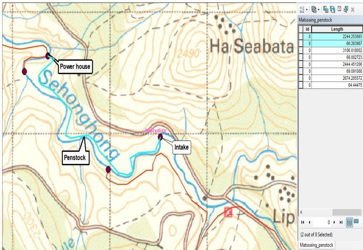
Figure 16: Contour lines and system layout for Matsoaing
