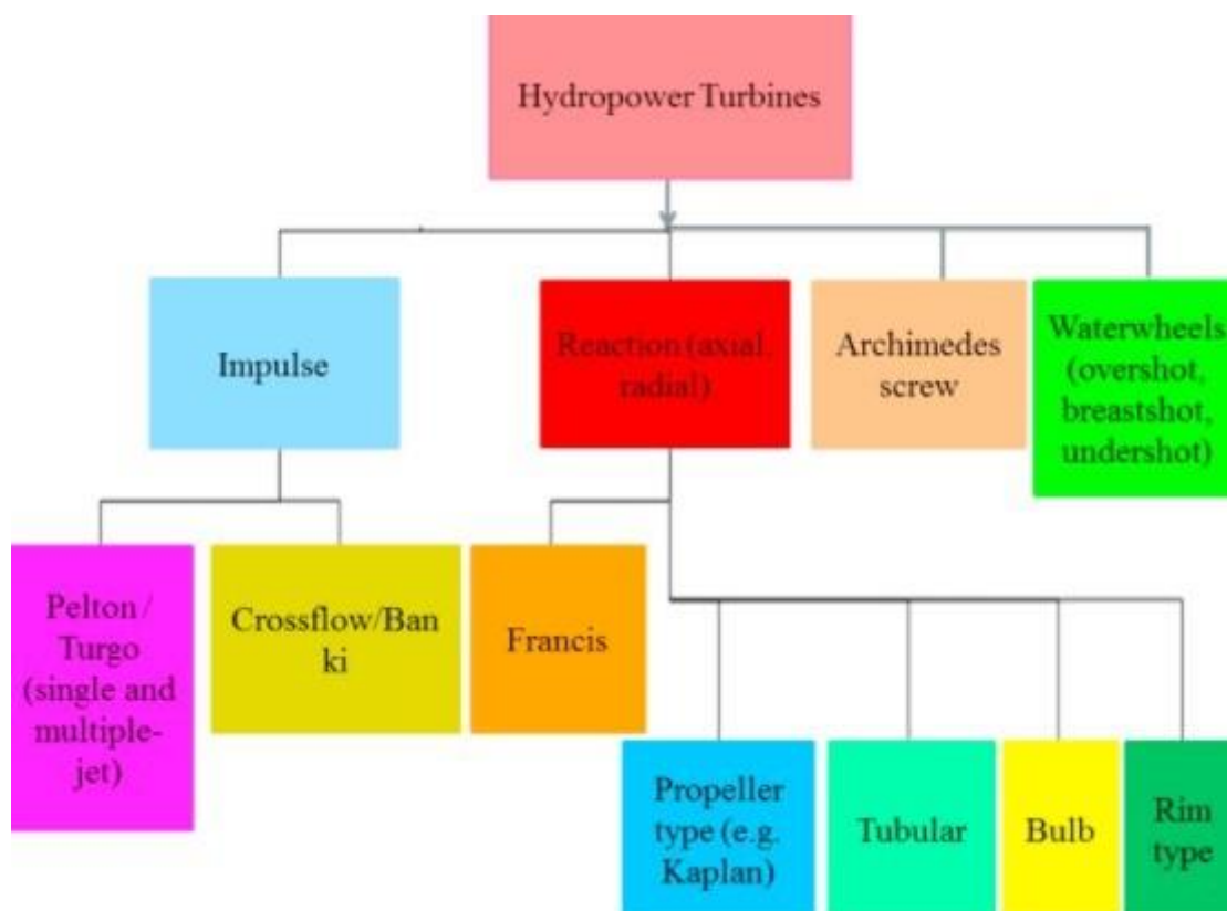
Figure 2: Turbine classification [25].
