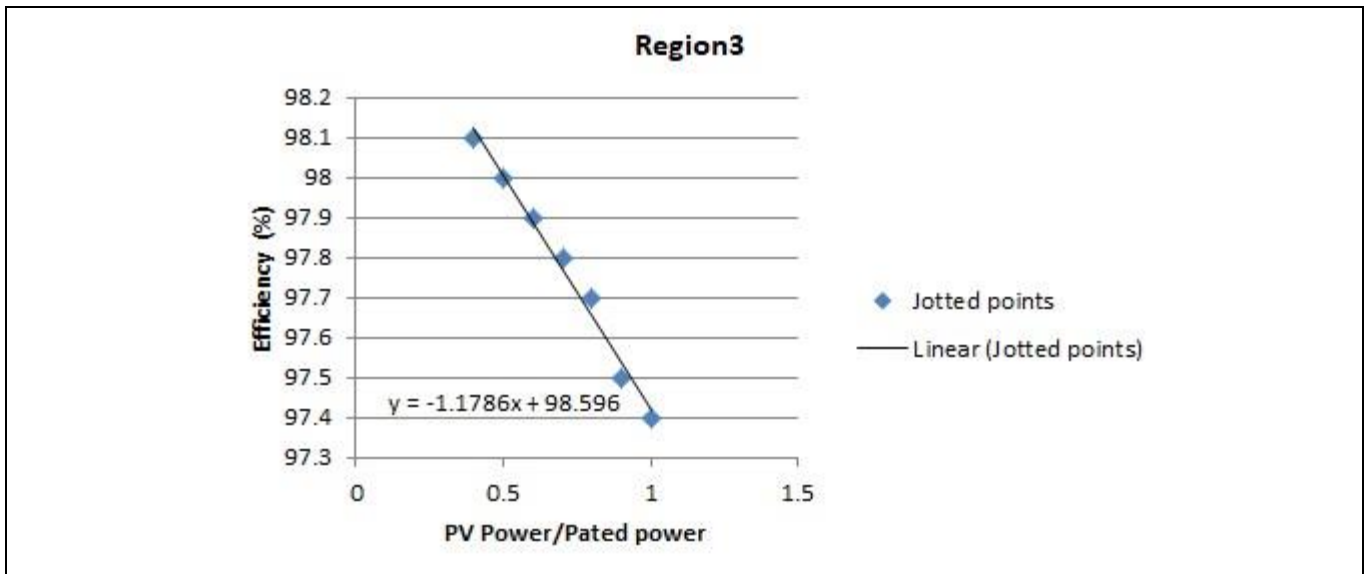
Figure 13: Regions describing the inverter efficiencies for commercial PV system
