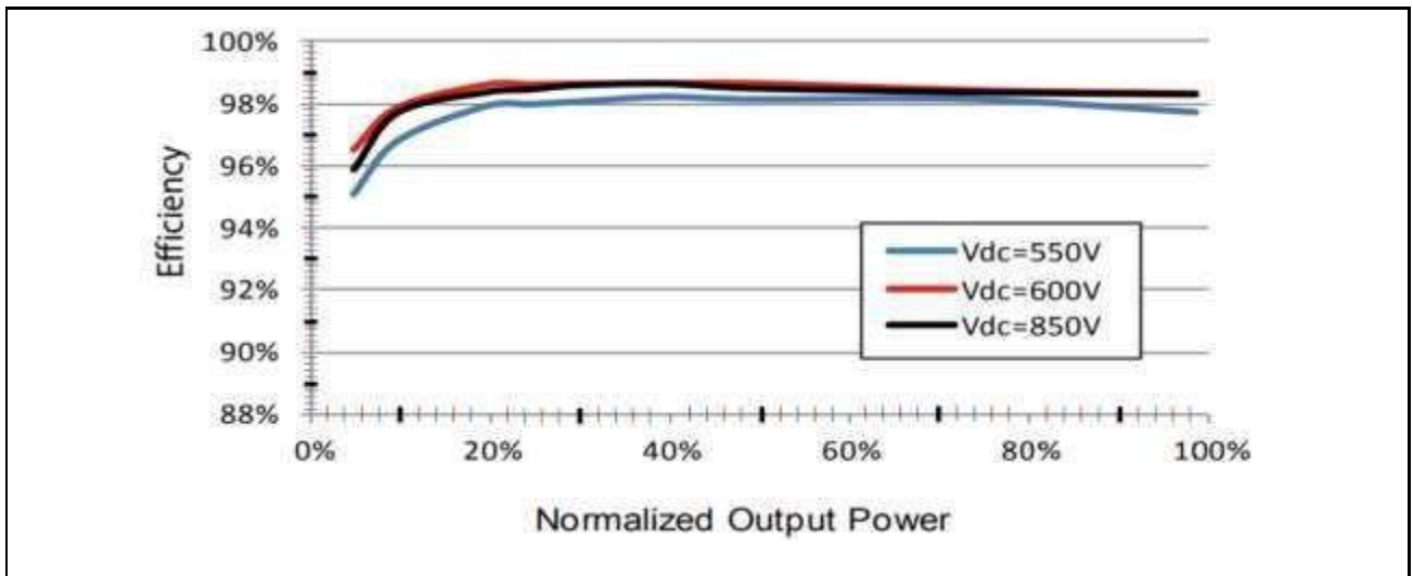
Figure 12: The inverter efficiency curves for commercial PV system
