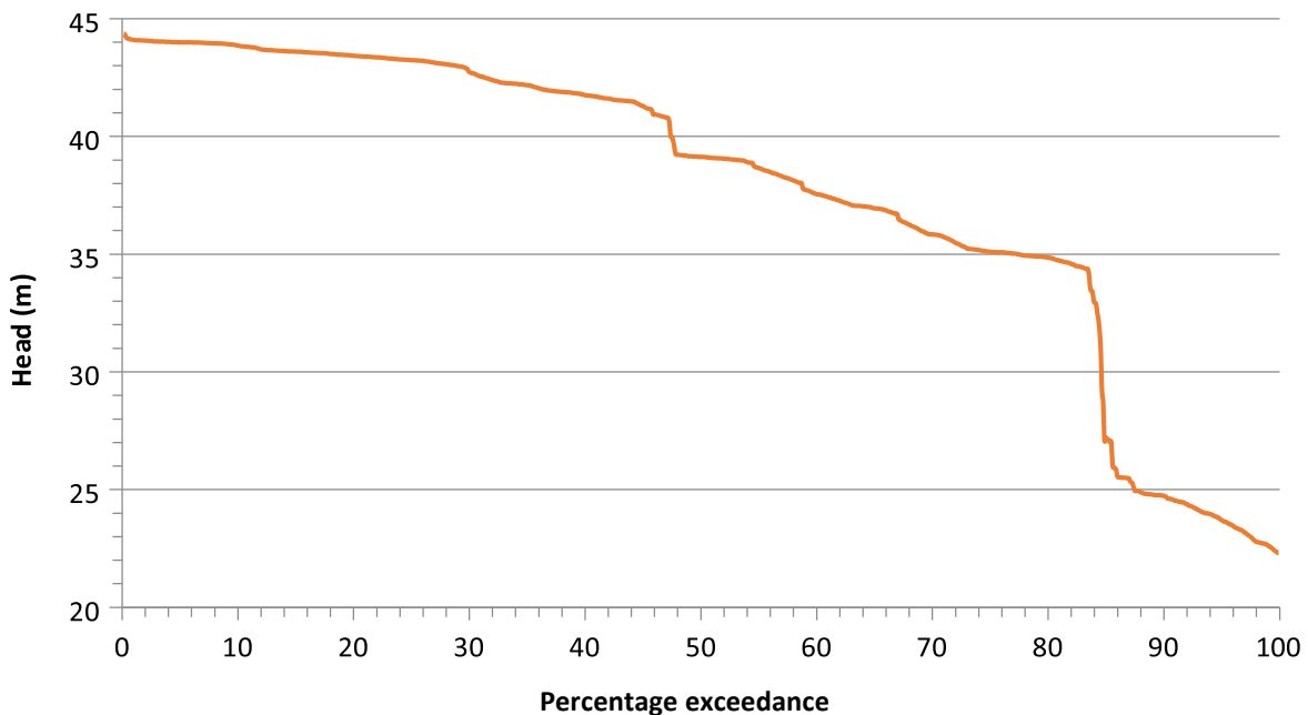
Figure 15: IFR head duration curve.
