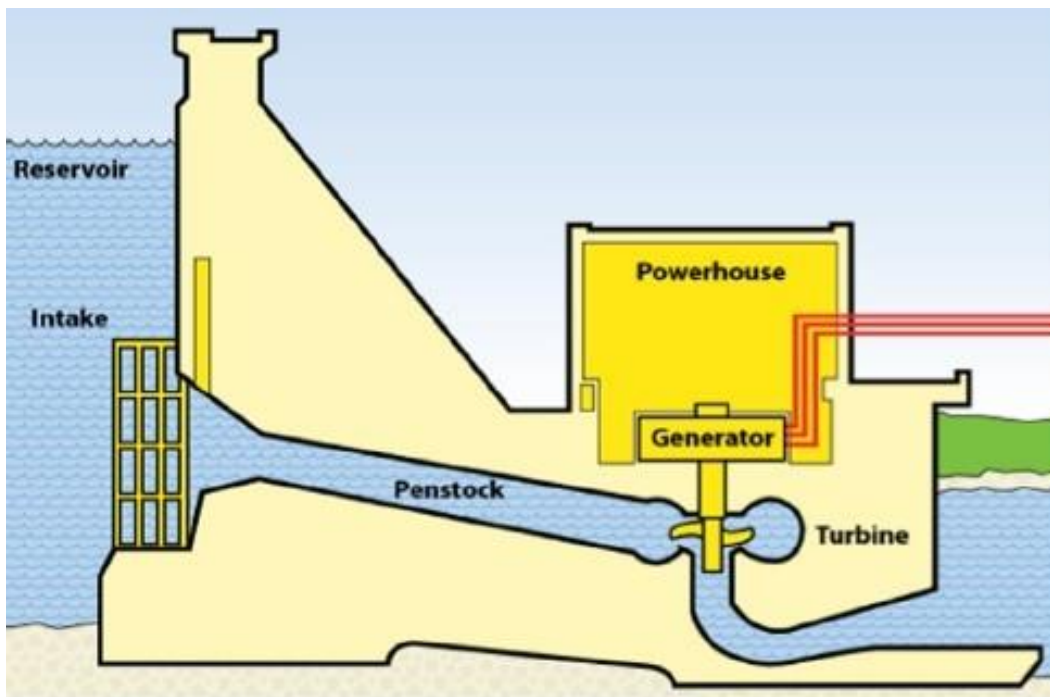
Figure 4 : Penstock integral with dam structure [69]
