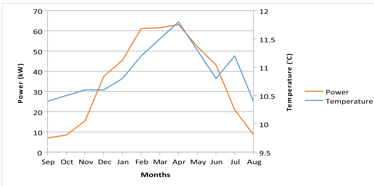
Figure 17: Power produced at IFR using actual water temperature and density for different months.
