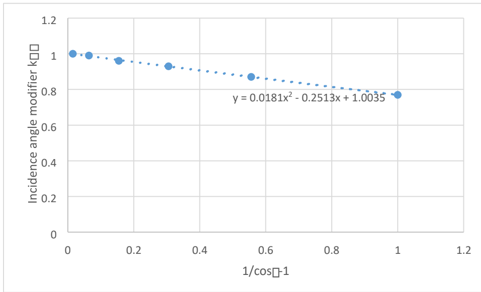
Figure 2: incidence angle modifiers for Sunmaxx collector
