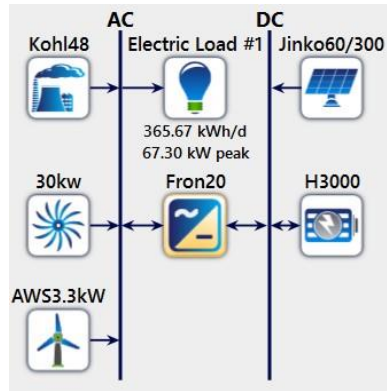
Fig 4.76 Solar/Hydro/Wind/Generator configuration
