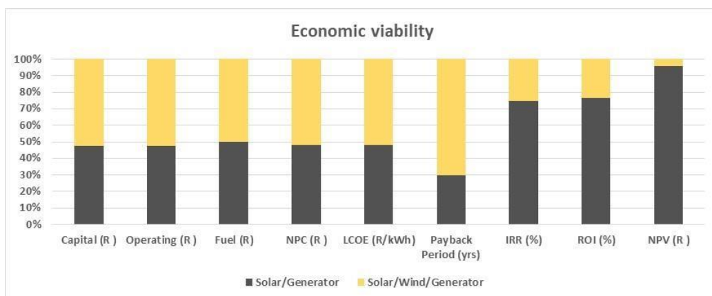
Fig 4.84 Economical values
