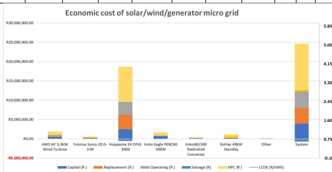
Fig 4.53 Solar/Wind/generator system Cost
