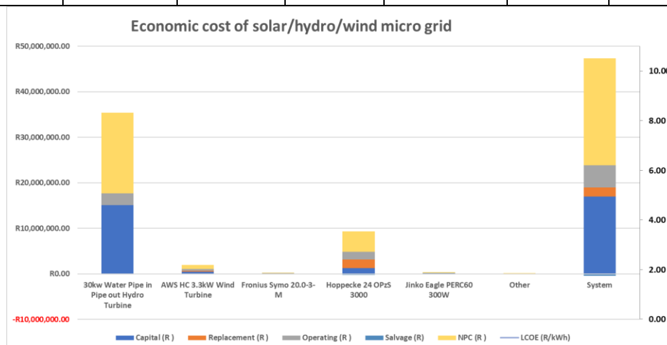
Fig 4.75 Solar/hydro/wind cost
