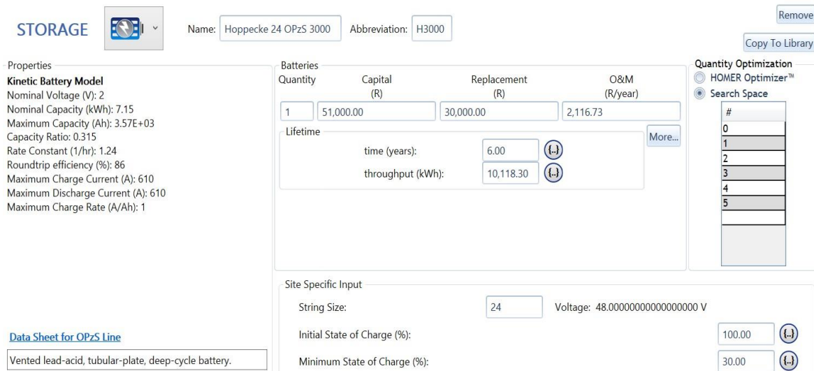
Fig 4.21 Search space of Hoppecke 24 OPzS 3000
