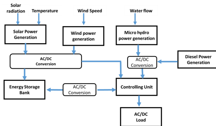
3.16 Solar/hydro/wind/generator hybrid micro grid
