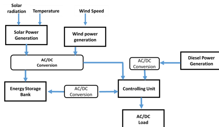
Fig 3.8 Solar/Wind/diesel generator hybrid micro grid
