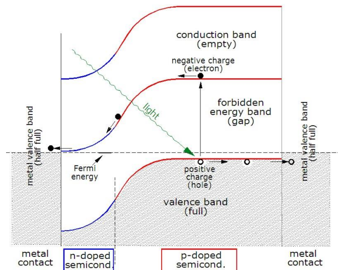
Fig 2.11 Photo-generation of Charge Carriers during Photovoltaic effect
