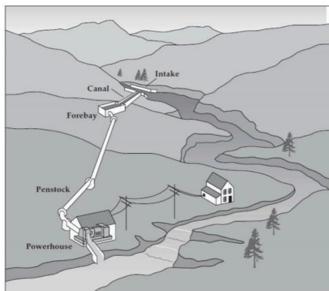
Fig 2.6 Layout of SHPP
