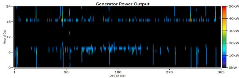
Fig 4.52 Diesel Generator Emissions
