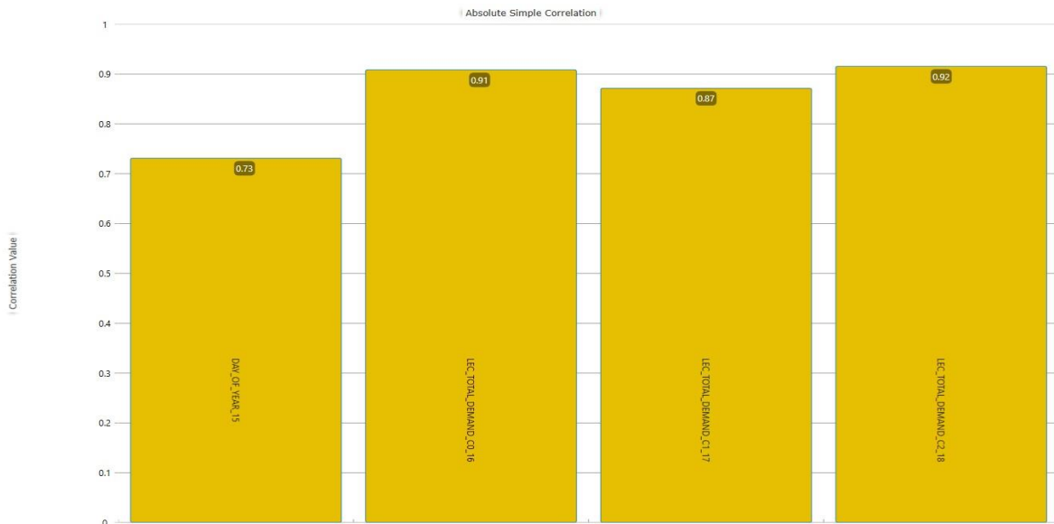
Figure 21 Correlation of Data from 2015 – 2018 for Hour-ahead (LEC_INTRADAY) Forecasting
