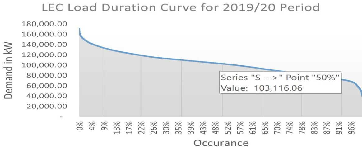
Figure 45 LEC Load Duration Curve for 2019/20 Period
