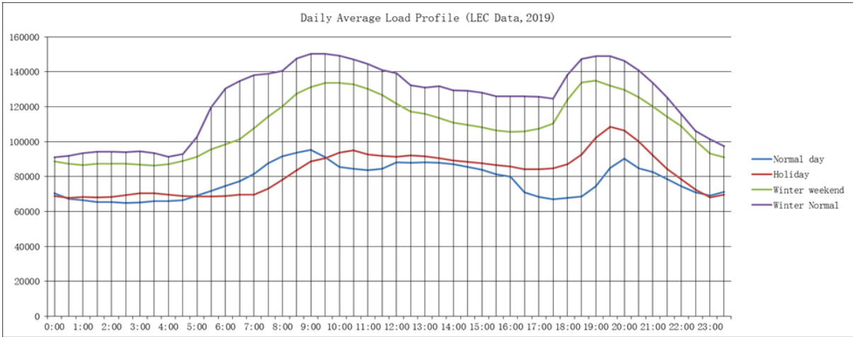
Figure 18 A 24 hour LEC Load Profile for Normal, Holiday and Winter Periods
