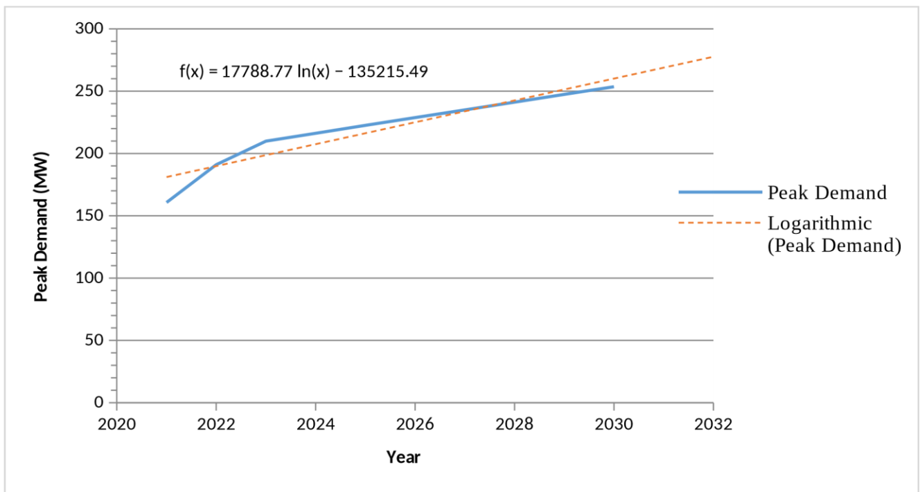
Figure 13: Average forecast electricity demand derived using logarithmic extrapolation
